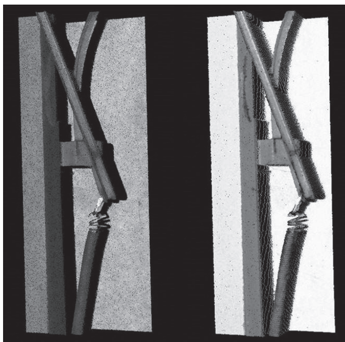
Figure 8: Image above shows objects scanned with TX8 on the left and another time-of-flight 3D scanner on the right, with ghost points between the two surfaces.
