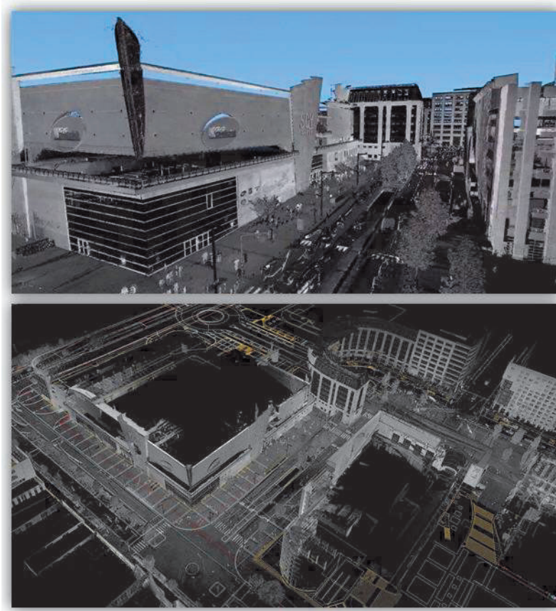
Figure 6: TX8 point clouds of urban environment
