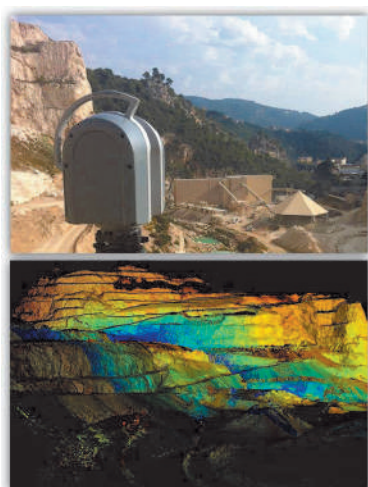
Figure 4: Quarry photo and point cloud of long range TX8 scan
