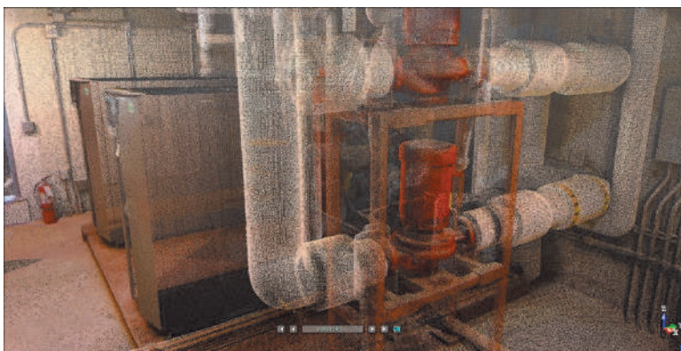
Figure 7: Colorized point cloud in RealWorks Station Based view
